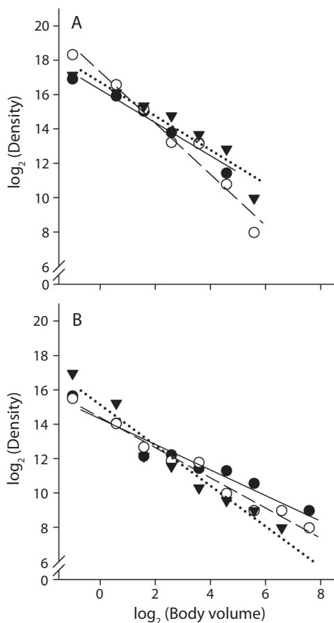
Fig. 3. Linearized body size spectra of shrimps (A) and snails (B) resulting from the multiple linear regression analyses conducted to determine differences in normalization constants and scaling exponents among the cold (solid circles-solid line), dry (empty circles-dashed line) and rainy (solid triangles-dotted line) seasons.
