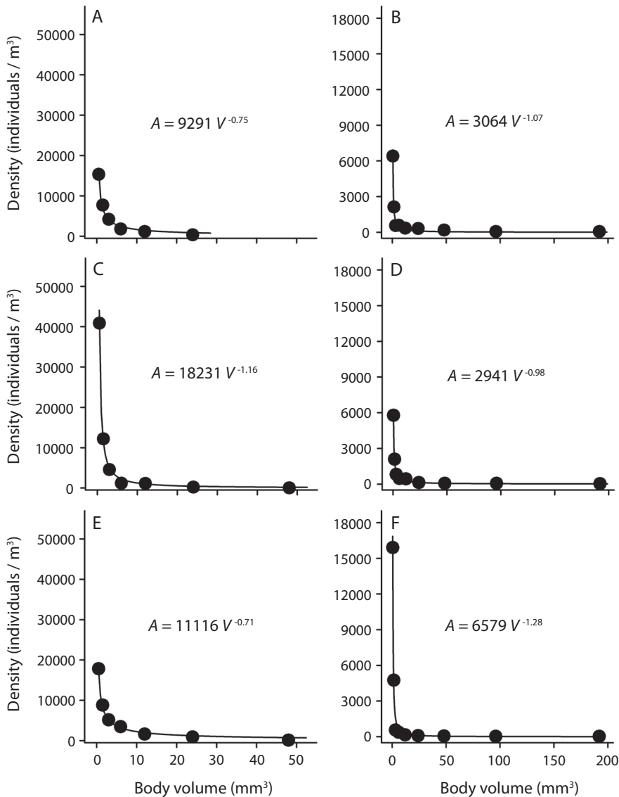
Fig. 2. Body size spectra of shrimps (left column) and snails (right column) estimated at the cold (A-B), dry (C-D) and rainy (E-F) seasons. The power functions describing these relationships between the density of individuals and the body volume are provided in the respective panel.
