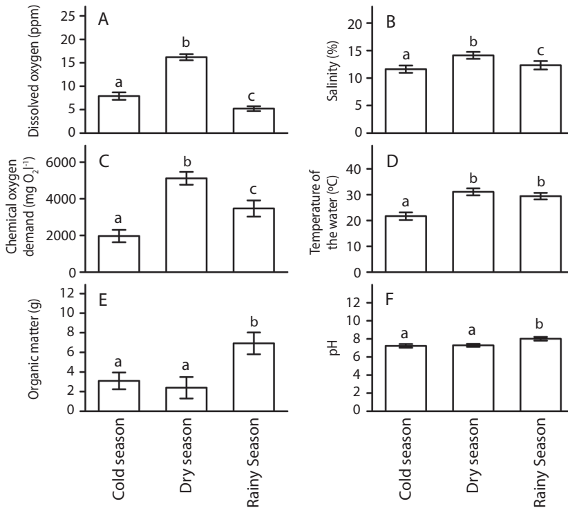
Fig. 1. Physicochemical variables (averages \pm 2 S.E.) measured at the cold, dry and rainy seasons in the Tamiahua Lagoon, Mexico, including dissolved oxygen (A), salinity (B), chemical oxygen demand (C), temperature of water (D), organic matter in sediments (E) and pH (F). Significant differences between seasons are indicated with different letters (Tukey test critical \alpha = 0.05 ).
