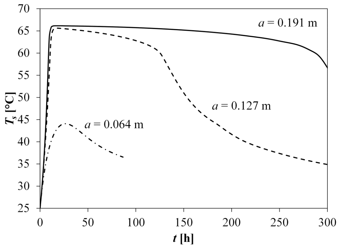
Fig. 6 Solid-liquid phase temperature at the center of the bioreactor as a function of changes in a
