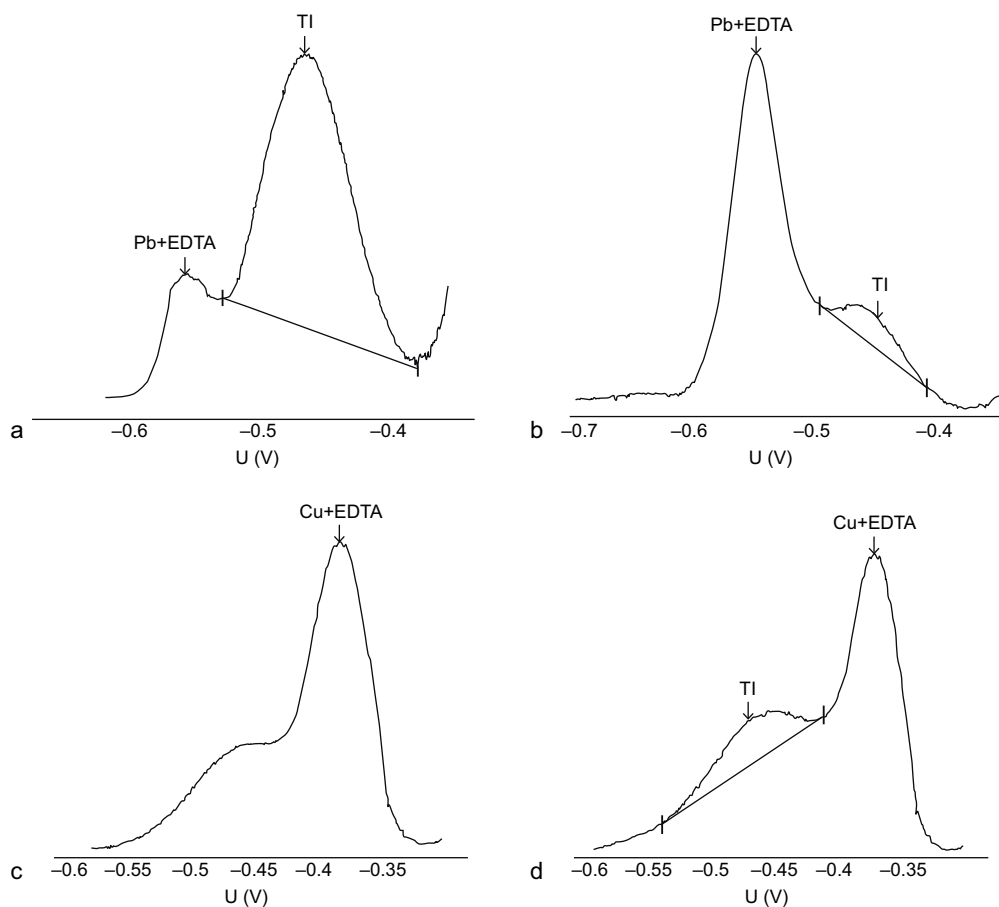
Fig. 2. Influence of the Pb(II) concentration: (a) 10 mg/L, (b) 20 mg/L, and Cu(II): (c) 5 mg/L, (d) 2 mg/L, in the differential pulse anodic stripping voltammetry (DPASV) potential (U) signal of 10 µg/L Tl(I) in the presence of 0.1 M ethylenediaminetetraacetic acid (EDTA). Intensity signal scales are arbitrary and vary among graphs. pH = 4.6. Deposition potential -0.700 V, deposition time 60 s, scan rate 20 mV/s, pulse amplitude 0.050 V
