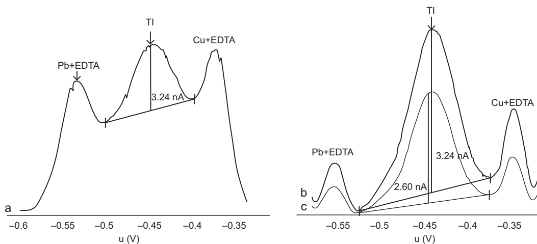
Fig. 5. Effect of deposition potential on the peak current of differential pulse anodic stripping voltammetry (DPASV) potential ( U ) signals for Tl(I), for 10 \mu\text{g/L} Tl(I) + 10 mg/L Pb(II) + 2 mg/L Cu(II) and 0.1 M ethylenediaminetetraacetic acid (EDTA), (a) from -0.700 to -0.600 V, (b) -0.550 V and (c) -0.500 V. Deposition time 30 s, scan rate 10 mV/s, pulse amplitude 0.050 V. Intensity scales are arbitrary
