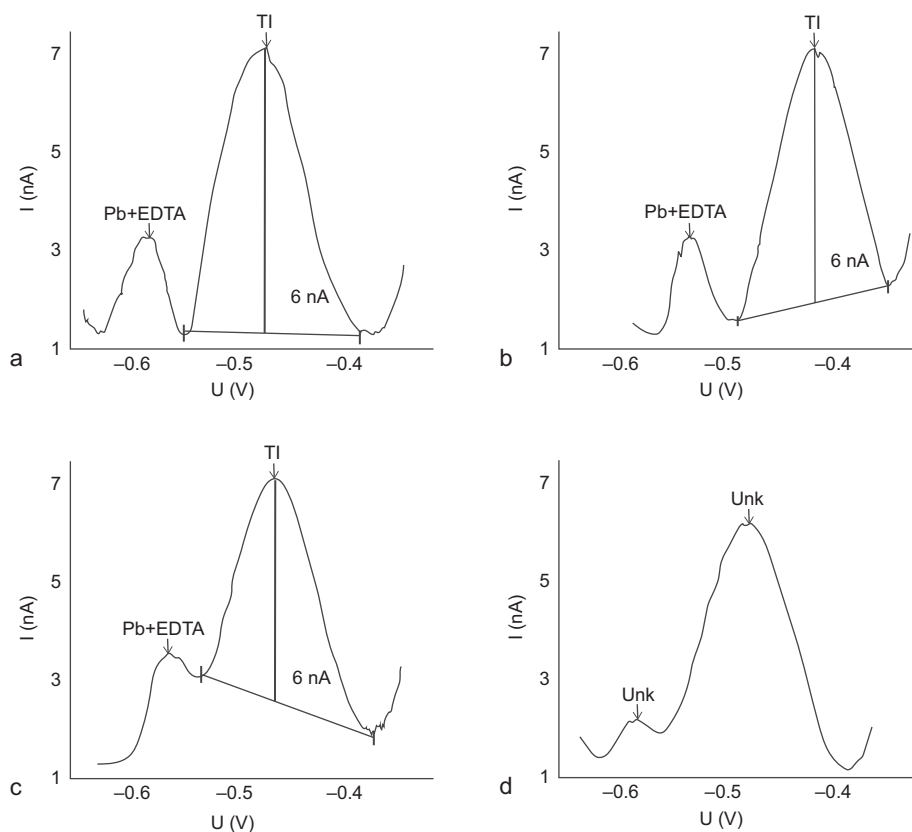
Fig. 3. Effect of the scan rate on the separation of differential pulse anodic stripping voltammetry (DPASV) potential (U) signals of Pb(II) + EDTA and Tl(I), 10 \mu\text{g/L} Tl(I) + 10 mg/L Pb(II) at 0.05 V pulse amplitude: (a) v = 5 mV/s, (b) v = 10 mV/s, (c) v = 20 mV/s, (d) v = 20 mV/s (0.07 V pulse amplitude). Deposition potential -0.700 V, deposition time 60 s, pulse amplitude 0.050 V in all, except 0.07 V in d
