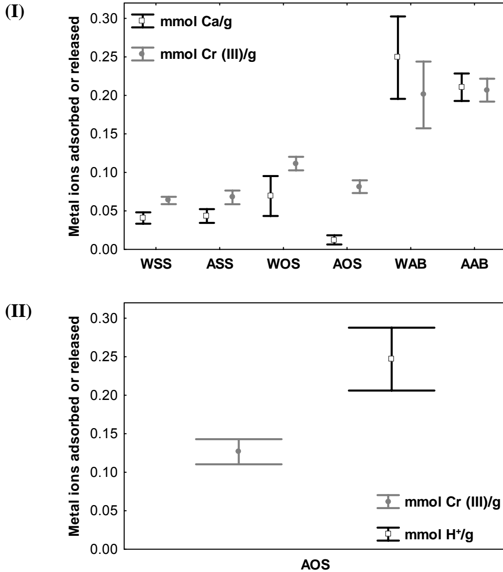
Figure 2.6 Metal ions adsorbed and released when agro-waste materials are used as adsorbents. (I) Chromium adsorbed and calcium released from water-washed and acid-washed agro-waste materials at pH 4, 25°C, and C_0=20 mg of Cr (III)/L. (II) Chromium adsorbed and H^+ released from acid-washed oats straw (AOS) without pH control at 25°C, initial pH 4, and C_0=120 mg of Cr (III)/L. Symbols represent the average values and bar errors were built with a confidence interval of 95%.
