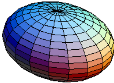
Figura 3.3: Elipsoide. Weisstein, Eric W. "Ellipsoid." From MathWorld--A Wolfram Web Resource. http://mathworld.wolfram.com/Ellipsoid.html
