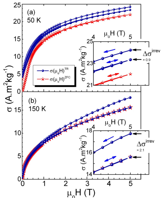
FIGURE 5. Demagnetization thermo-remnant curve \sigma(\mu_0 H)^{TR} followed by the subsequent field-up and field-down \sigma(\mu_0 H) curves (blue circles), measured at T_{meas} = 50 K and 150 K. For the sake of comparison, the magnetization curves for both increasing and decreasing the magnetic field measured from the demagnetized state \sigma(\mu_0 H)^{ZFC} are also plotted (red stars). Insets: zoom into the high-field region of the curves to indicate the irreversible magnetization change \Delta\sigma(\mu_0 H)^{irrev} (the value given is in \text{Am}^2\text{kg}^{-1} ). Arrows indicate whether the magnetic field is being increased or decreased.
