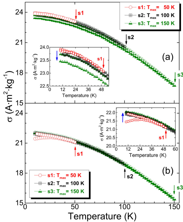
FIGURE 4. (a) Effect of the successive thermal cycling between 10 K and T_{max} (for T_{max} = 50 K, 100 K, and 150 K) on the \sigma(T) curve at \mu_0 H = 5 T after field-cooling (a), and zero field-cooling (b), from 350 K. Insets: zooms into the low temperature region of the curves.
