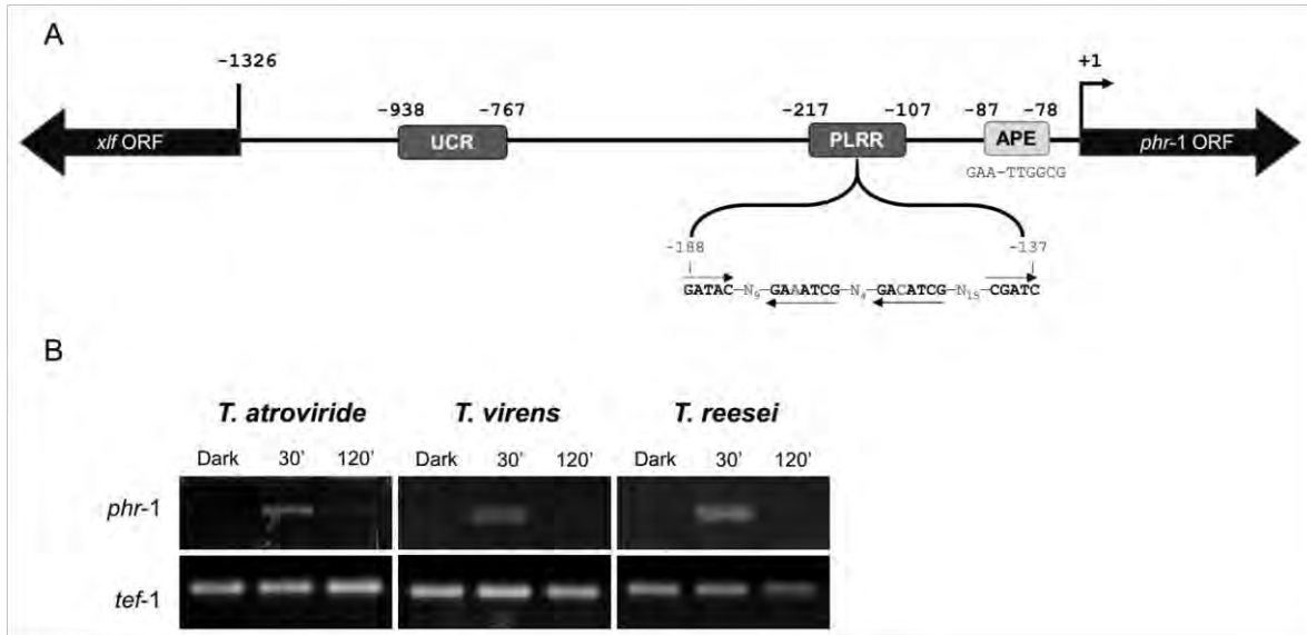
Figure 1. Promoter elements of the photoinducible gene phr-1 are conserved among Trichoderma spp. (A) Schematic representation of phr-1 gene promoter architecture, which resulted from T. atroviride , T. virens , T. reesei , T. citrinoviride , and T. longibrachiatum phr-1 promoter sequence alignment (Fig. S1). The upstream conserved region (UCR) and the Potential Light Response Region (PLRR) are depicted by dark grey rectangles. The PLRR contains two inverted CGATN-boxes between the GATA-1 and -2 boxes of the core LRE. The albino proximal element (APE) is shown as a light grey rectangle. The phr-1 open reading frame (ORF) and the putative upstream xlf ORF are indicated in black solid arrows. Location and sequence of potential cis acting elements on the promoter are indicated below rectangles for each. Bold numbers on top represent the location of the different elements along the promoter from the transcriptional start site (+1) (thin arrow). (B) RT-PCR analysis of T. atroviride , T. virens , and T. reesei phr-1 gene expression under dark (control), or 30 and 120 min after a blue light pulse. Elongation factor 1 ( tef-1 ) gene was used as housekeeping control gene.
